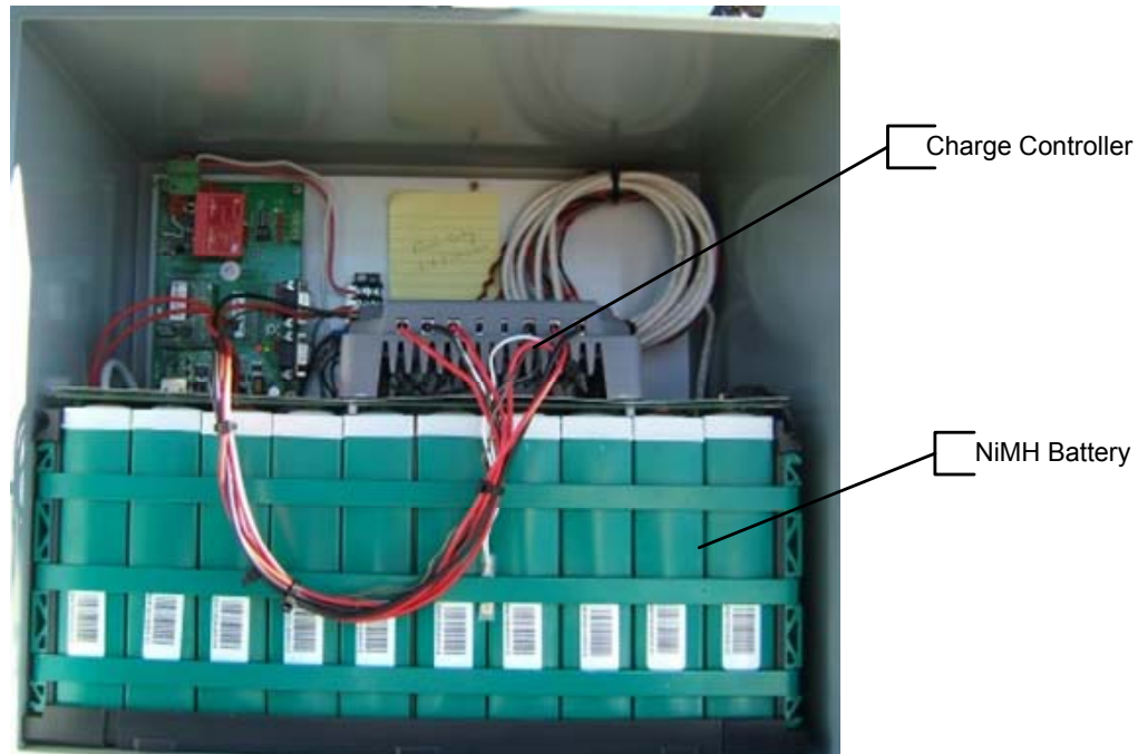
Figure 4 – Test Configuration #1 NEMA 4 Cabinet with NiMH Battery and Built-In Charge Controller
