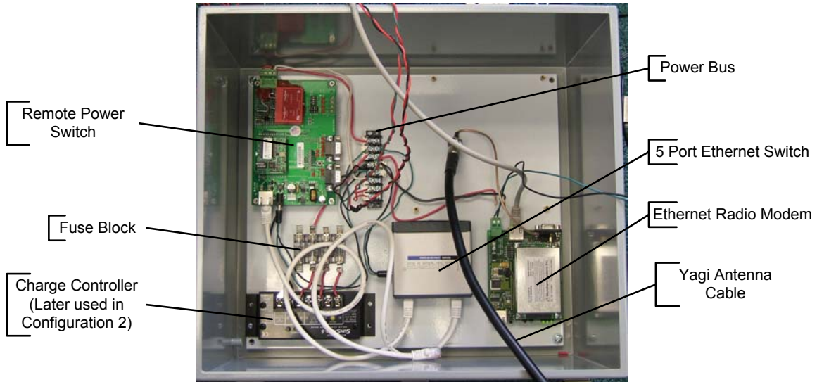
Figure 3 – Test Configuration #1 Hardware
