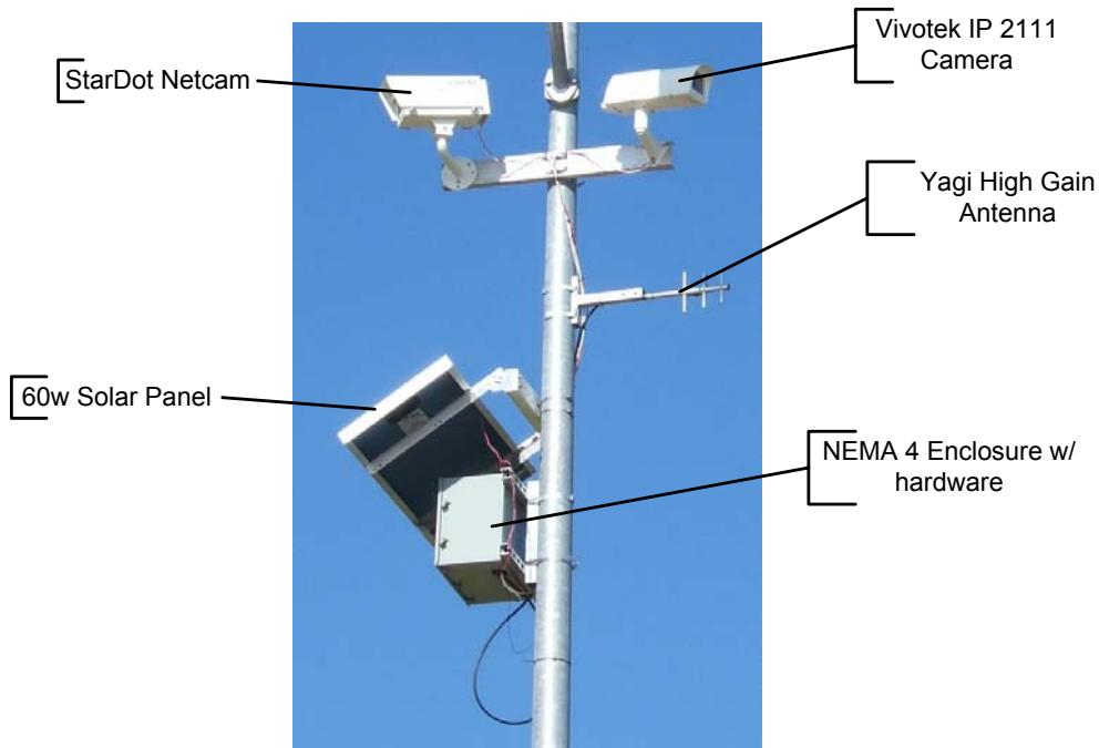
Figure 2 – Test Configuration #1
