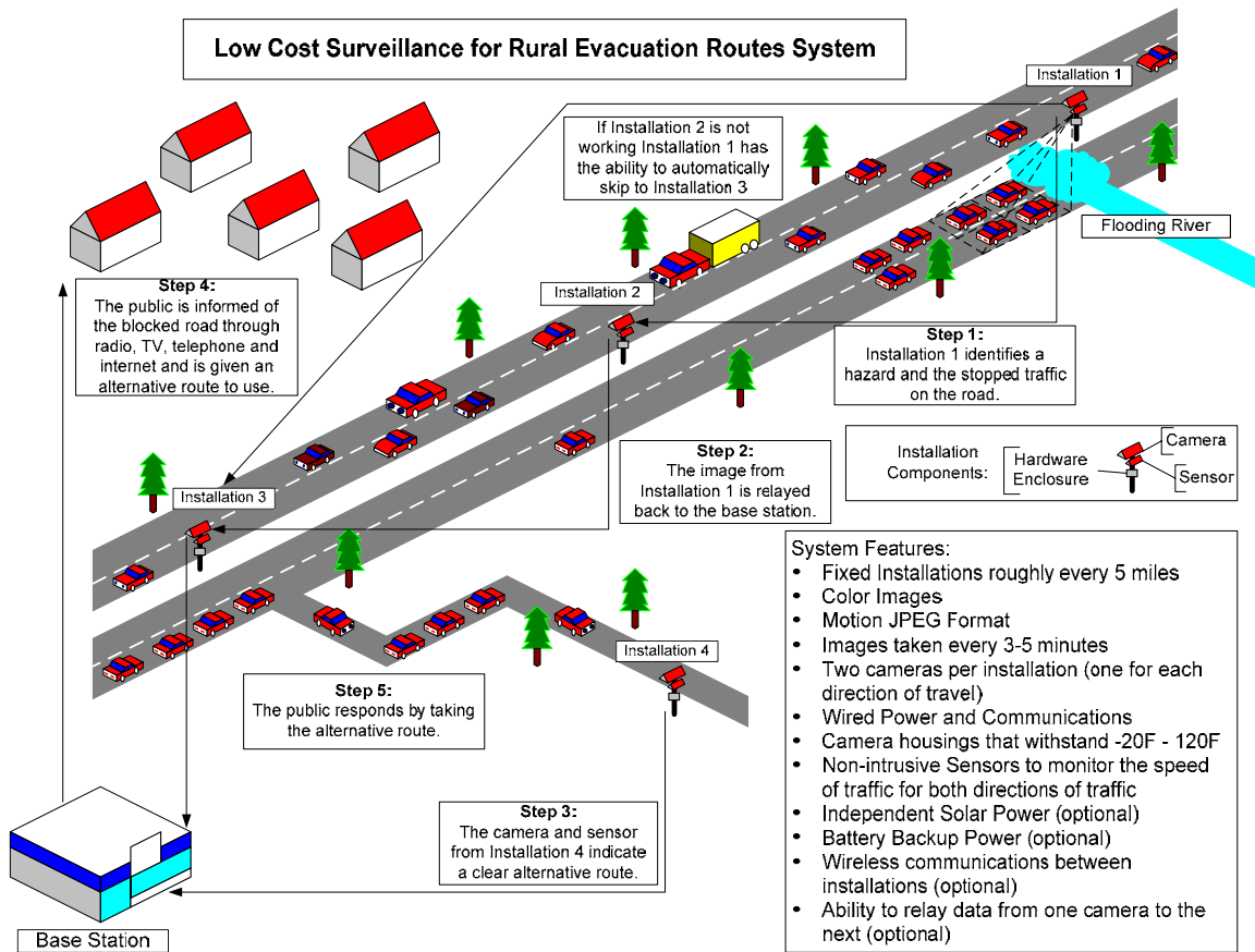
Figure 1 – Rural Evacuation System Overview
