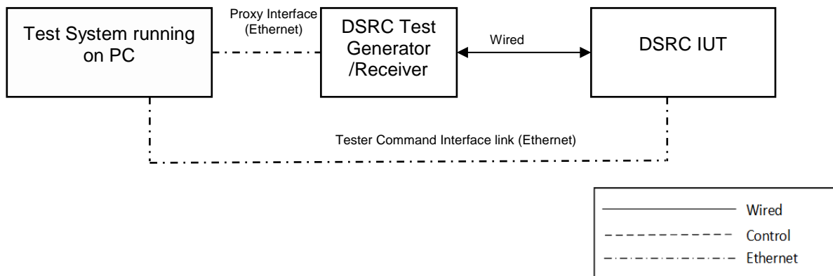
Figure 4: Test Configuration 4 (TC4)
